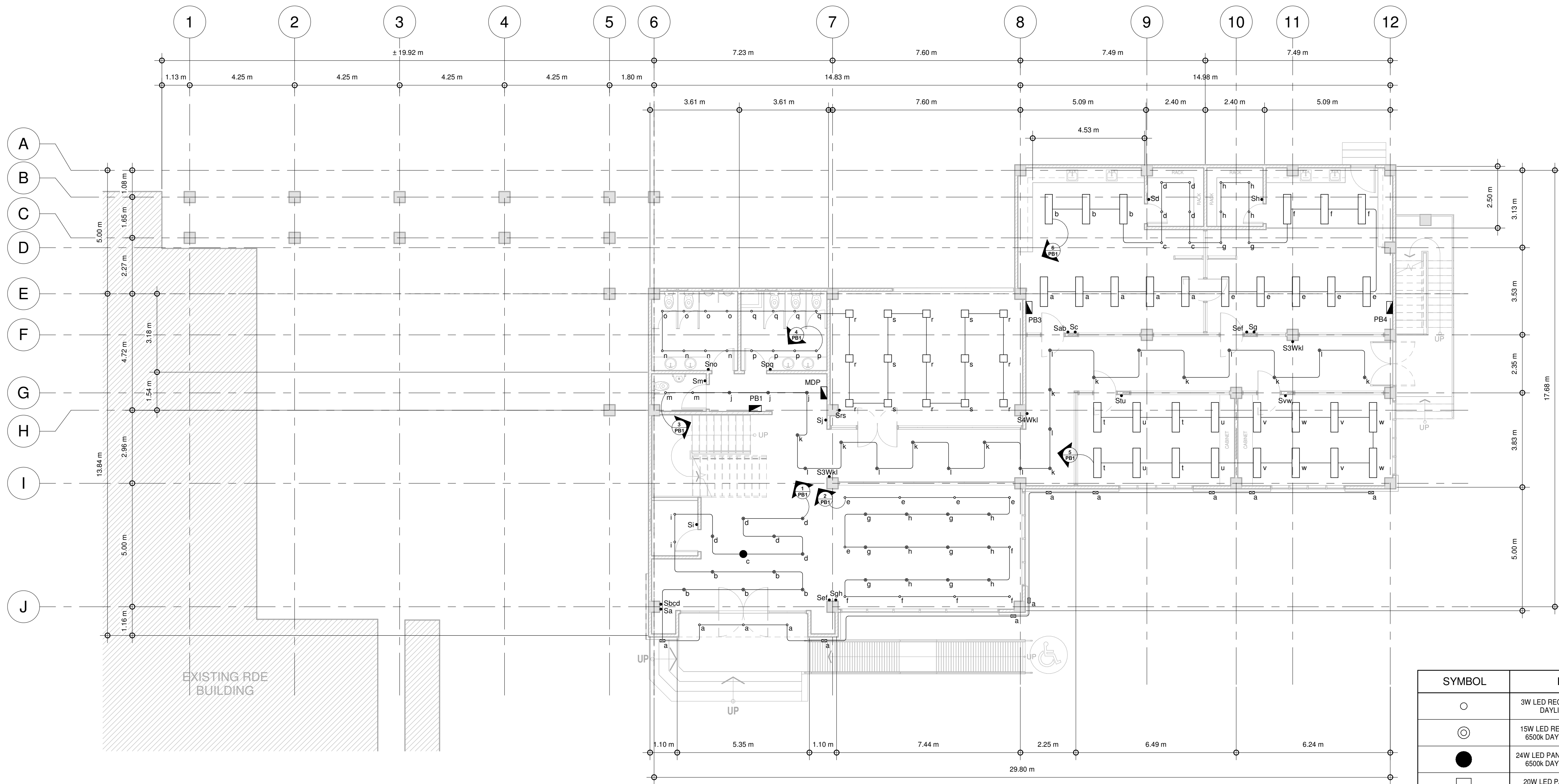
1 GROUND FLOOR LIGHTING LAYOUT PLAN 1 : 100 meters
